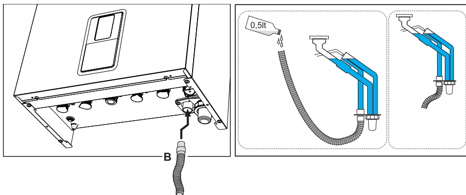
fig. 52- Condensate drain connection
