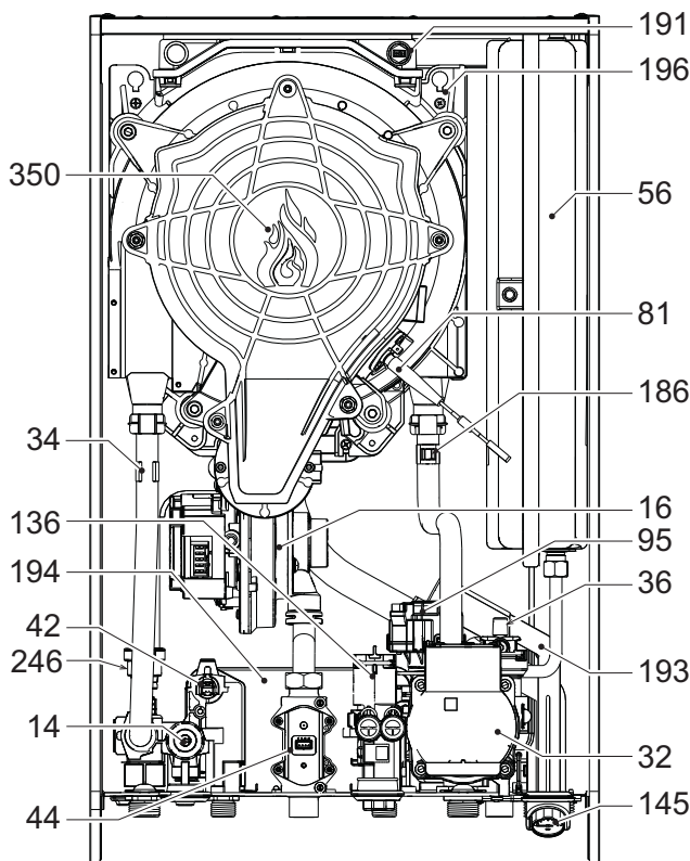
fig. 77- General view
