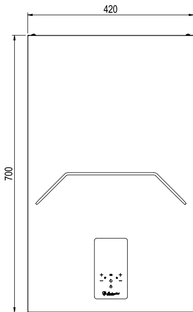
fig. 73- Front view
