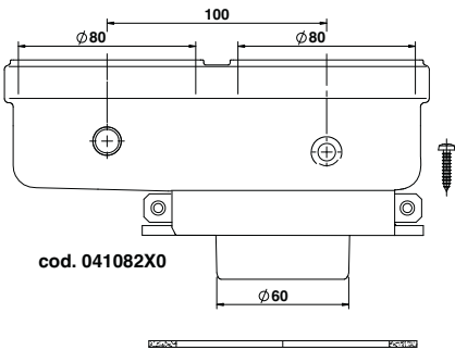
fig. 36- Starting accessory for separate ducts
