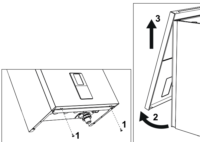
fig. 56- Front panel opening
