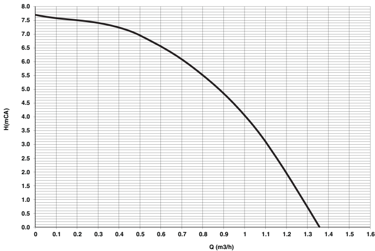
fig. 80- Residual head available for system
