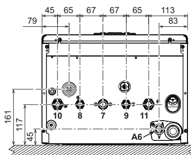
fig. 76- Bottom view
