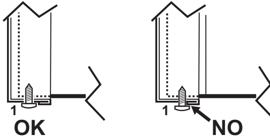
fig. 57- Correct position of front panel
