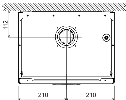
fig. 75- Top view
