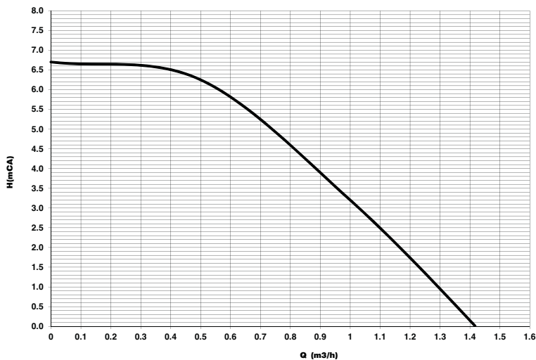
fig. 79- Residual head available for system
